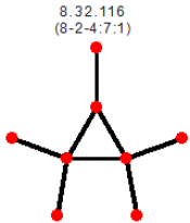
Homeomorphism class 8.32 (8-2-4:7): 1 graph
