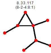
Homeomorphism class 8.33 (8-2-4:8): 1 graph
