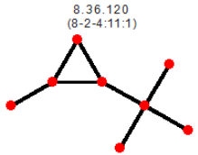
Homeomorphism class 8.36 (8-2-4:11): 1 graph
