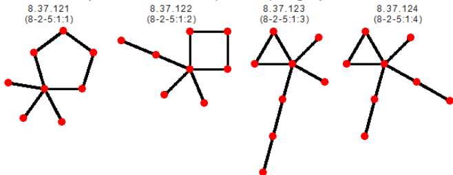
Homeomorphism class 8.37 (8-2-5:1): 4 graphs
