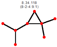
Homeomorphism class 8.34 (8-2-4:9): 1 graph
