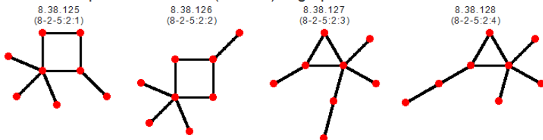
Homeomorphism class 8.38 (8-2-5:2): 4 graphs
